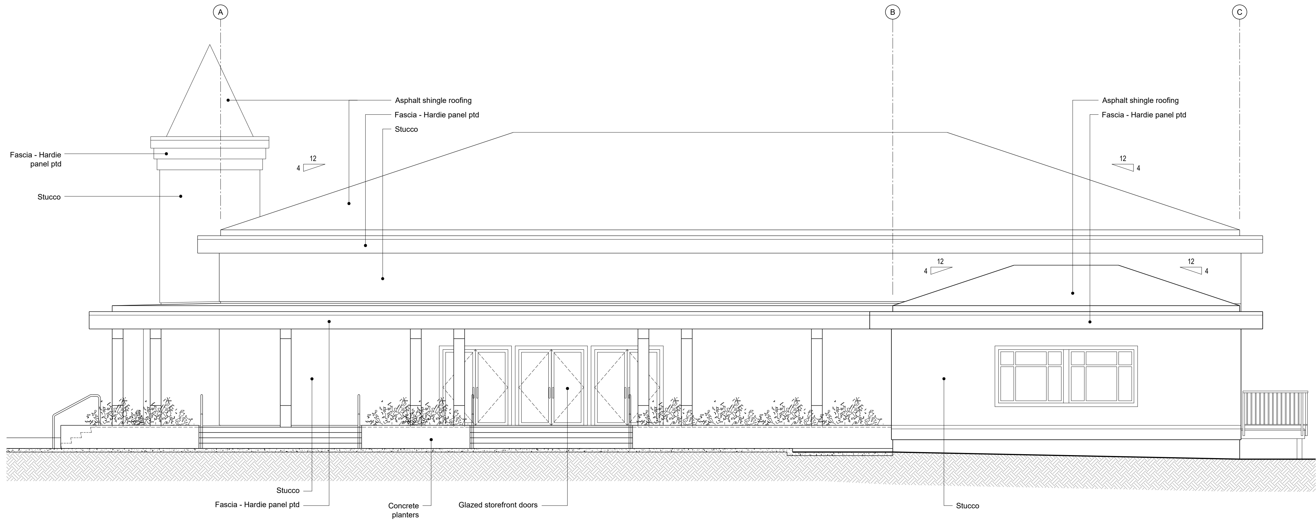
2 A2.12 South Elevation 3/16" = 1'-0"
