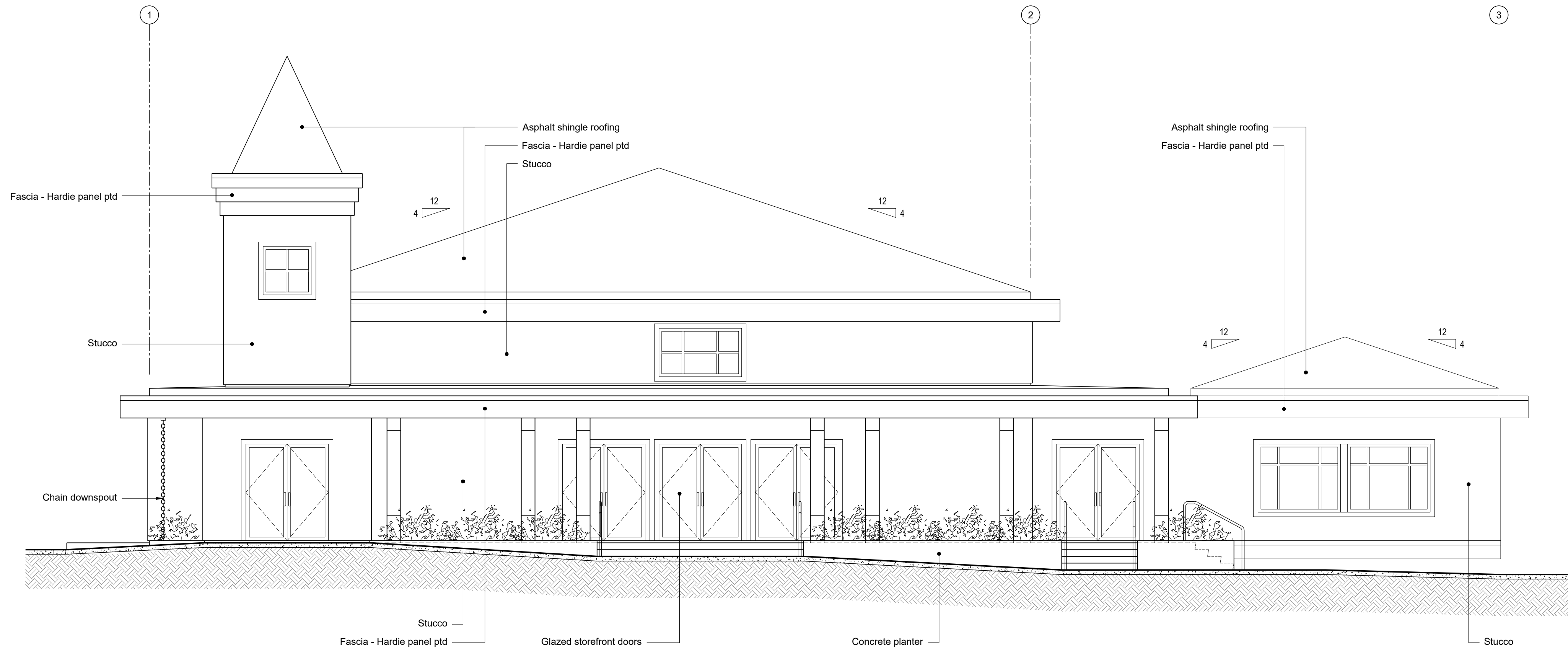
1 A2.12 West Elevation 3/16" = 1'-0"
